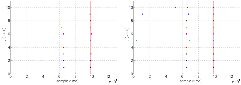
Fig. 2. Change point candidates at each scale, with vertical lines at the true change positions. Left: DWT-SIC at J=10 levels, db2 , \alpha = 10^{-2} , n_{min} = 256 . Right: SWT-SIC at J=10 levels, db2 , \alpha_{j=1,\dots,10} = [10^{-1} \ 10^{-2} \ 10^{-3} \ 10^{-4} \ 10^{-5} \ \dots \ 10^{-5}] , n_{min_{j=1,\dots,10}} = [256 \ 1024 \ 4096 \ 16384 \ 65536 \ \dots \ 65536] .
