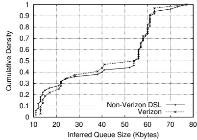
Fig. 8. Verizon-Non-Verizon: Inferred Access Queues
