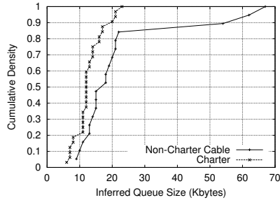
Fig. 7. Charter-Non-Charter: Inferred Access Queues
