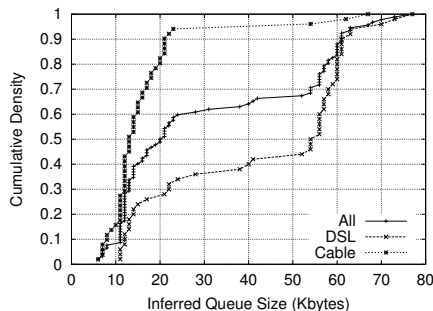
Fig. 6. Cumulative Density Functions of Access Queue Size Inferred by QFind
