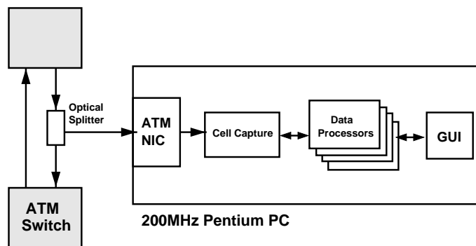
Fig. 3. The architecture of the ATM monitor.
