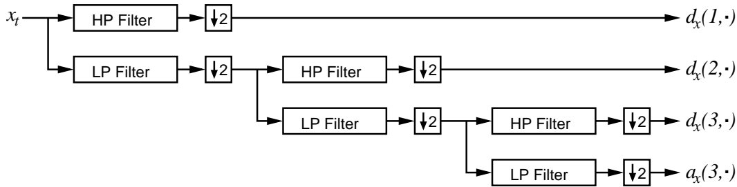
Fig. 2. The filter-bank. At each level in the recursive structure, the High Pass (HP) output: d_x(j, \cdot) , and the Low Pass (LP) output: a_x(j, \cdot) , occur at half the rate of the input a_x(j-1, \cdot) .
