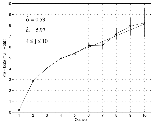
Fig. 1. An example of the Logscale Diagram for a LRD process with strong SRD. The vertical bars at each octave give 95% confidence intervals for the y_j . The series is simulated FARIMA(0,d,2) with d = 0.25 ( \alpha = 0.50 ) and \Psi = [-2, -1] implying c_f = 6.38 . Selecting (j_1, j_2) = (4, 10) allows an accurate estimation despite the strong SRD: \hat{\alpha} = 0.53 \pm 0.07 , \hat{c}_f = 6.0 with 95% confidence intervals 4.5 < \hat{c}_f < 7.8 .
