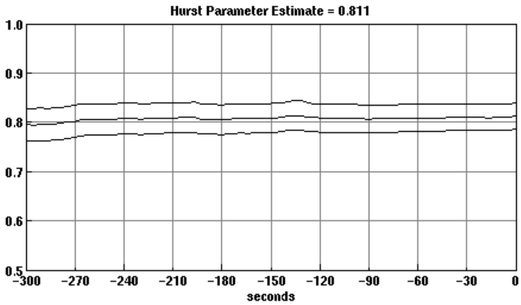
Fig. 6. An example output of Hurst parameter estimation. The three curves shown are, in order from the top, the upper 95% confidence interval, the estimate, and the lower 95% confidence interval.
