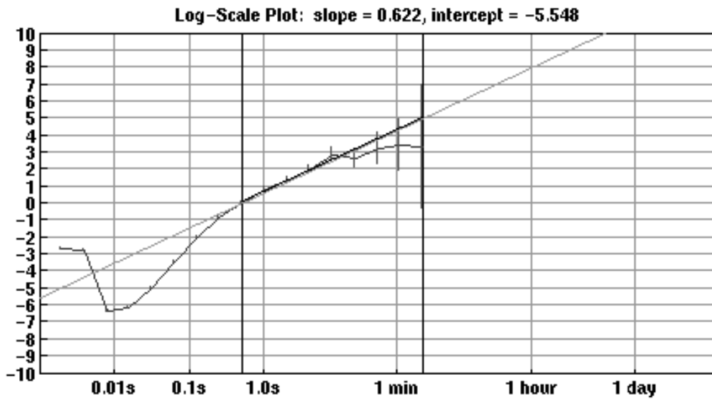
Fig. 7. The Logscale Diagram for the generated traffic showing a fitted regression line, and the scales used in the regression (shown as vertical lines across the entire y -range).
